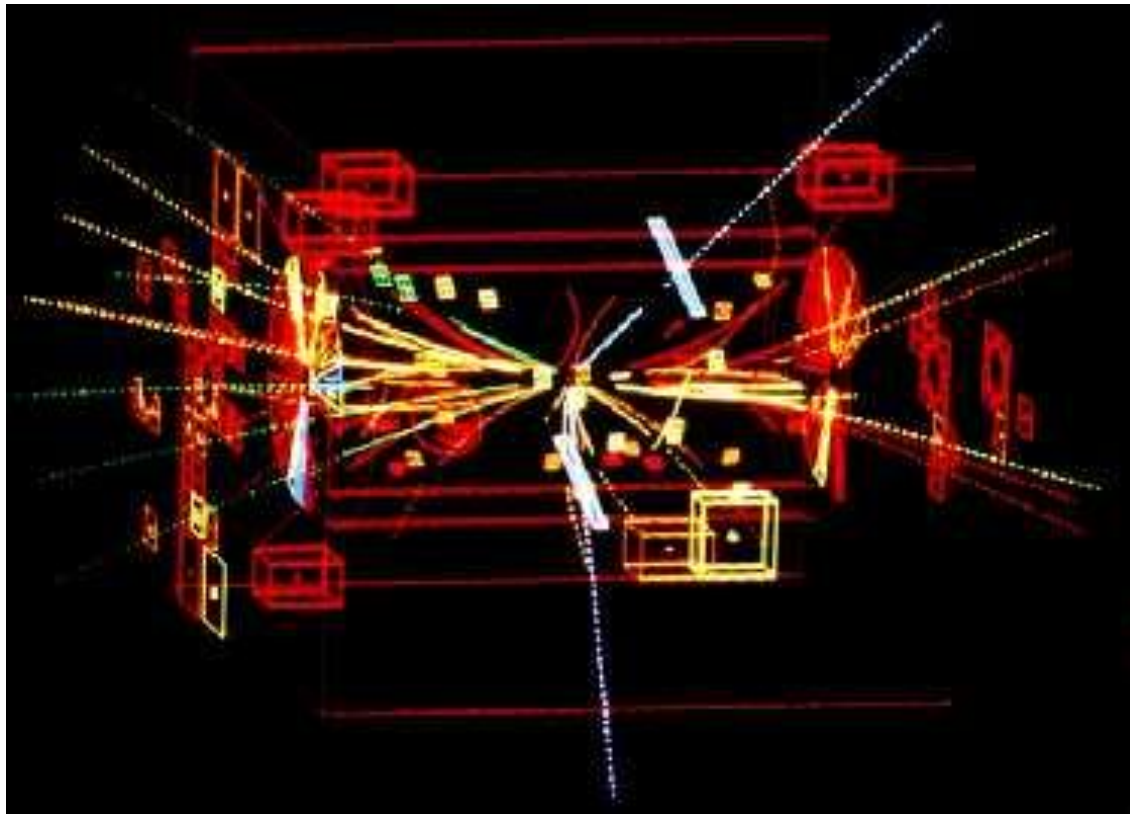
Z-Discovery at UA1 CERN in 1984
