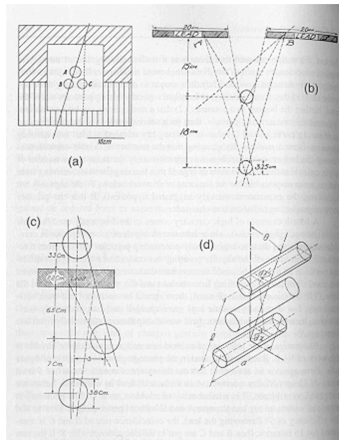
Early coincidence counting experiment
