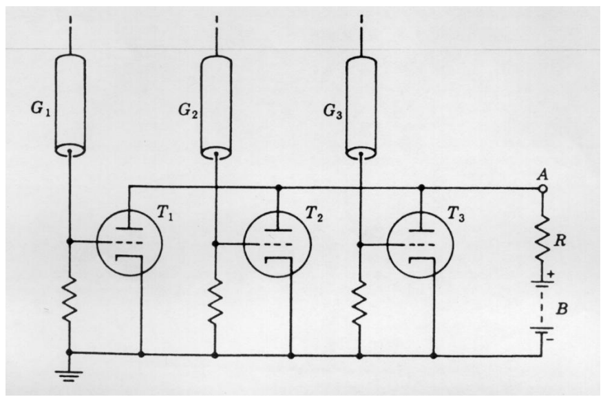
Rossi 1930: Coincidence circuit for n tubes
